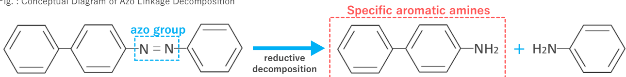
Fig. : Conceptual Diagram of Azo Linkage Decomposition
